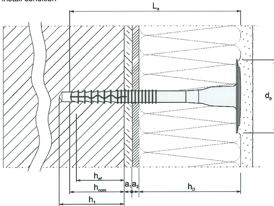
Anchor in its install condition
